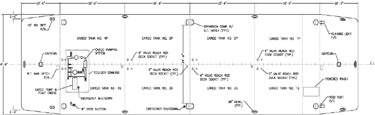
MAIN DECK PLAN M.T.S.
