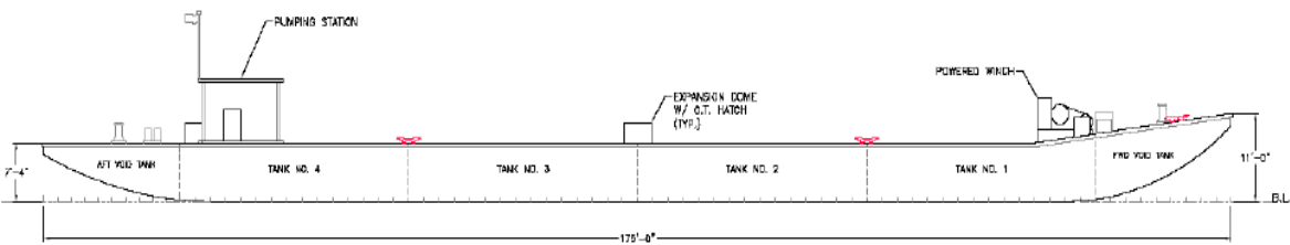
OUTBOARD PROFILE
