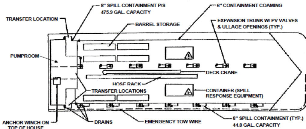
180-2 DECK PLAN
