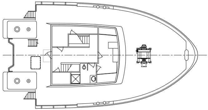
FOC'SLE DECK
