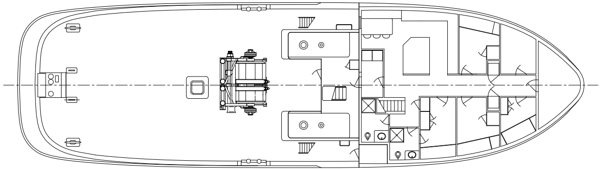
MAIN DECK
