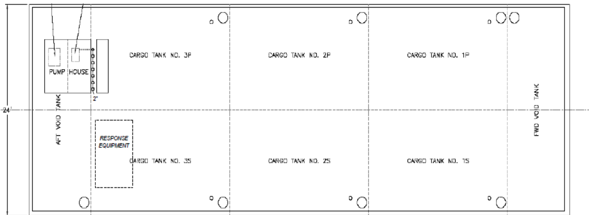
MAIN DECK PLAN 3/8" = 1'-0"
