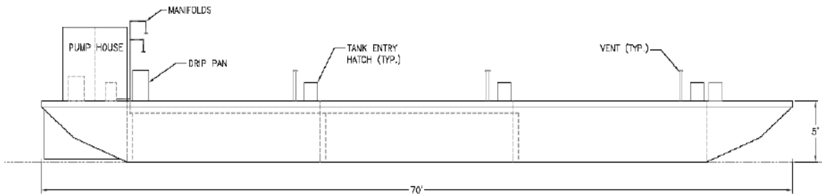
OUTBOARD PROFILE
